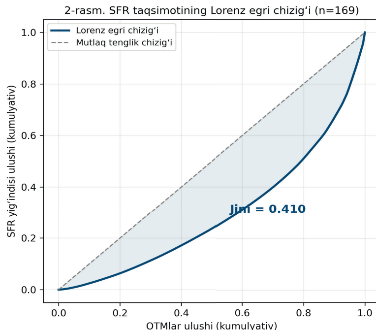
2-rasm. SFR taqsimotining Lorenz egri chizig'i (n=169). Manba: muallif hisob-kitoblari.
