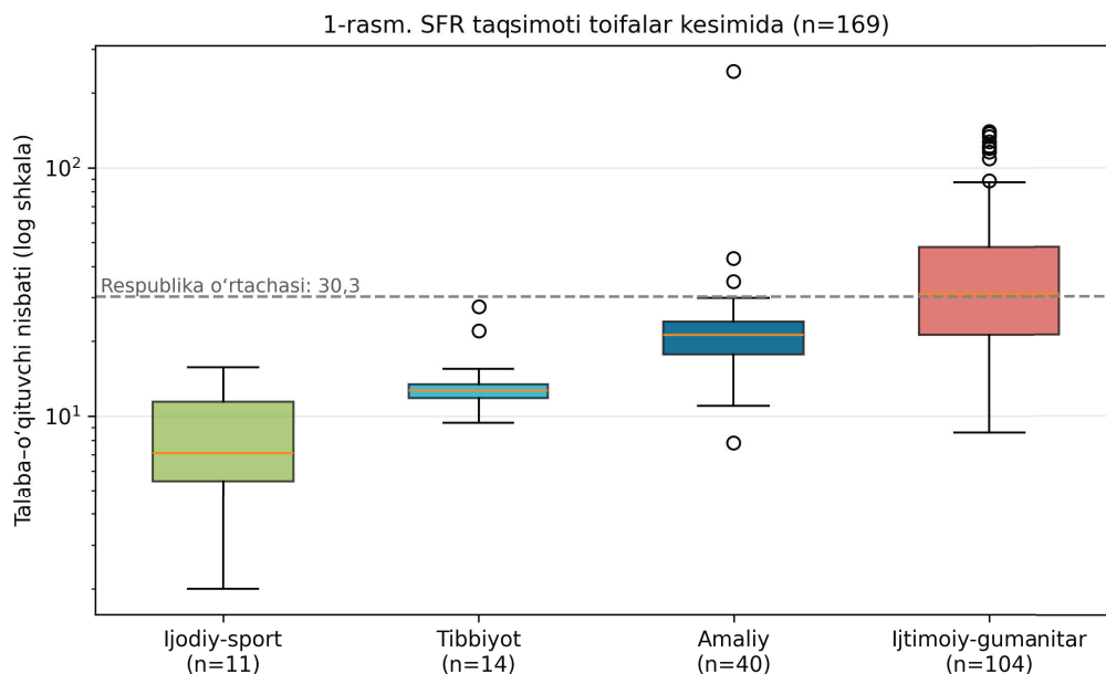
1-rasm. SFR taqsimoti toifalar kesimida (logarifmik shkala). Manba: [4] asosida muallif tomonidan tuzilgan.
