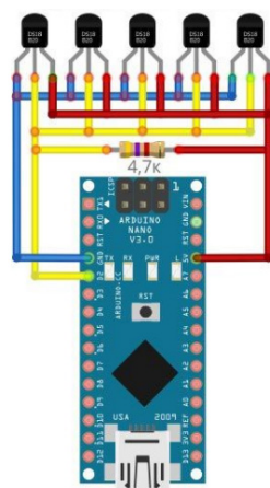
4-rasm. Bir nechta DS18B20 termosensordlarning 1-wire shinasini yordamida bitta Arduino Nano mikrokontrolleriga ulanish sxemasi
