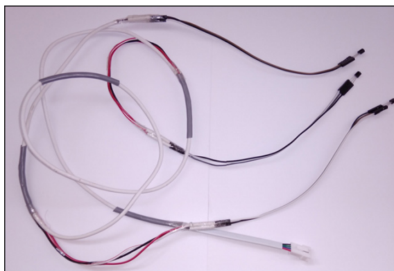
2-rasm. Bitta kabelga parallel ulangan termosensorlar shinasi
