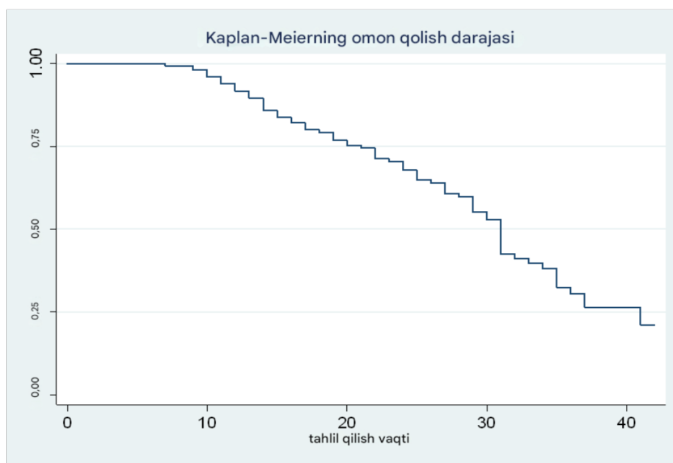
2-rasm. Kaplan Meier omonlik modeli
