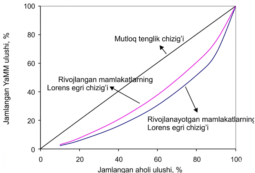
1-rasm. Lorens egri chizig'i 1
